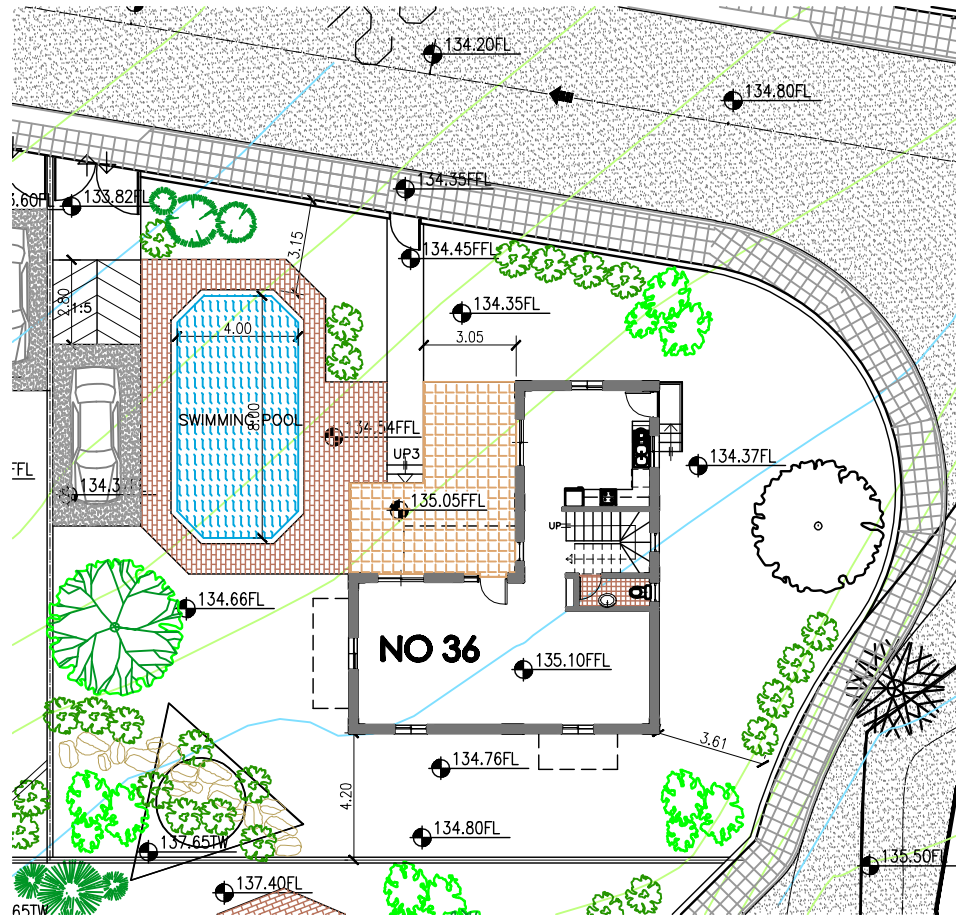
LAYOUT PLAN
