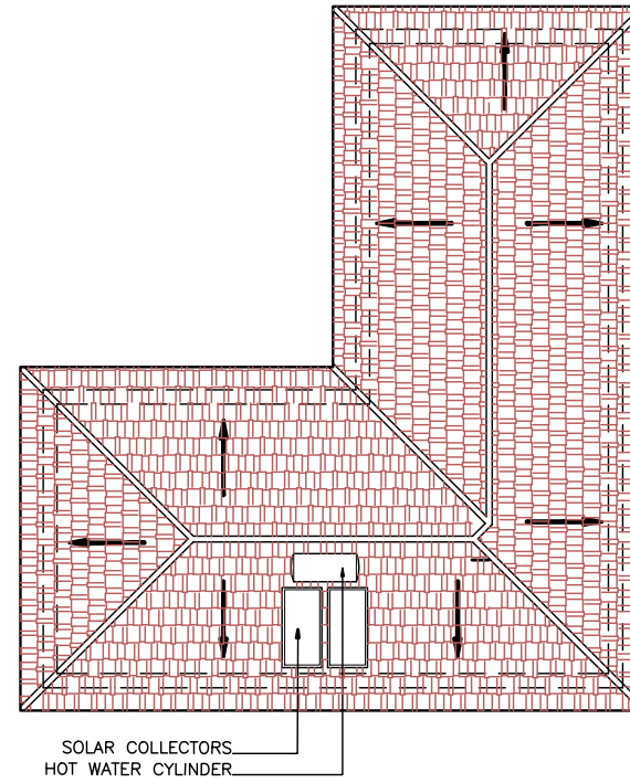
ROOF PLAN
