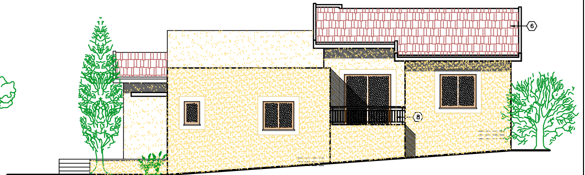
SIDE ELEVATION
